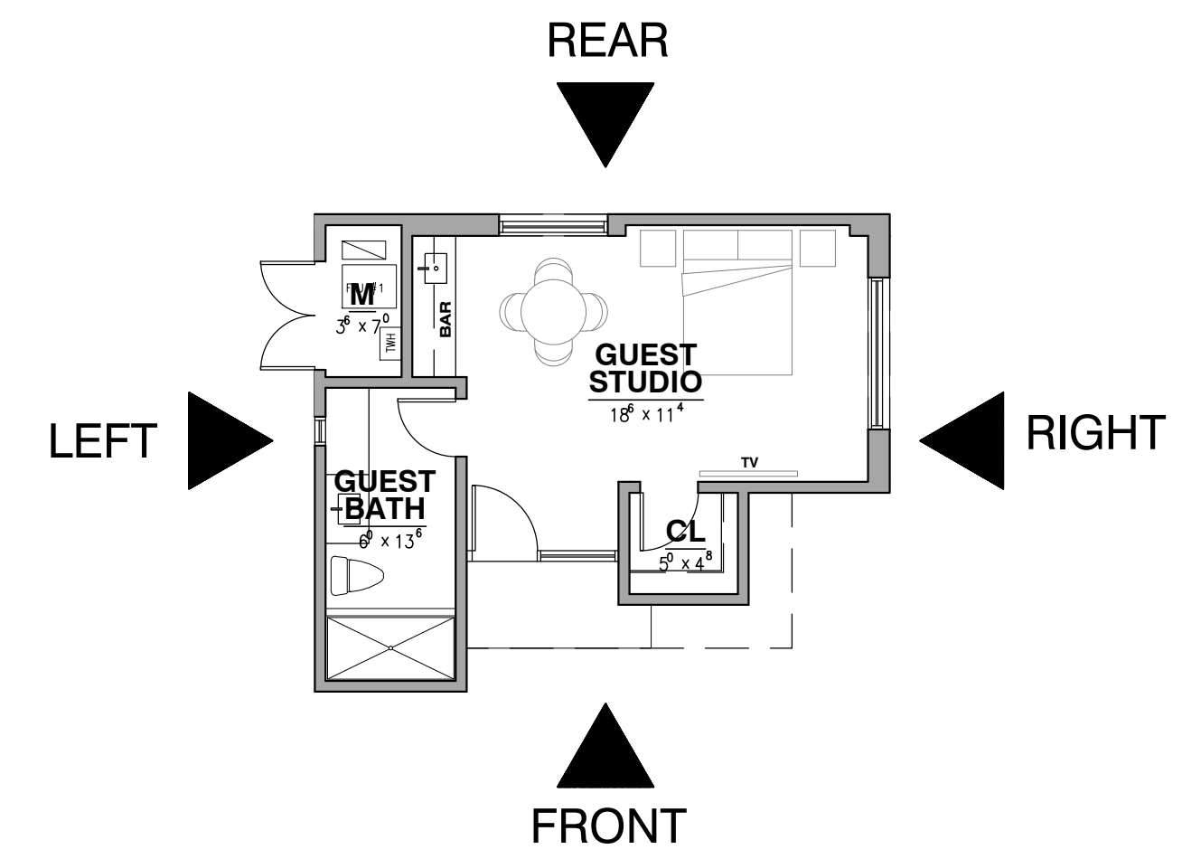
GUEST HOUSE 424 CONCEPT FLOOR PLAN
