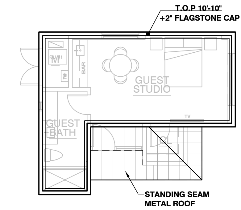
GUEST HOUSE 424 CONCEPT ROOF PLAN
