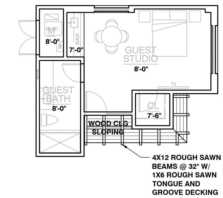
GUEST HOUSE 424 CONCEPT REFLECTED CEILING PLAN
