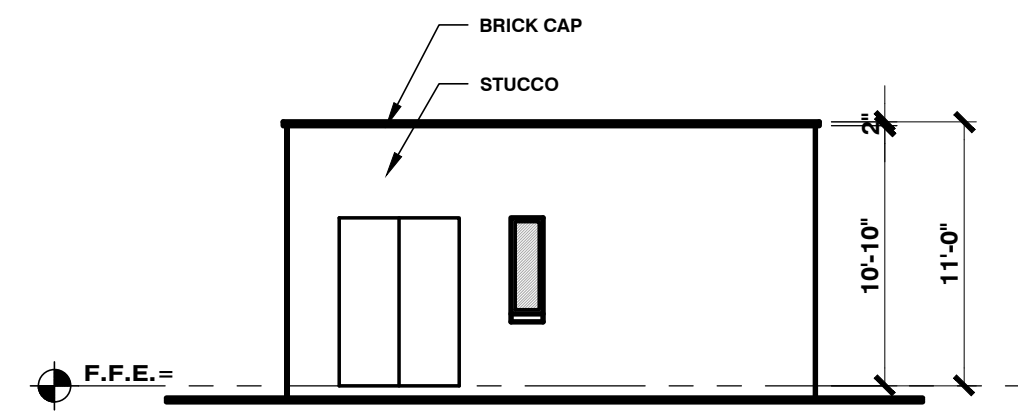
GUEST HOUSE 424 LEFT ELEVATION
