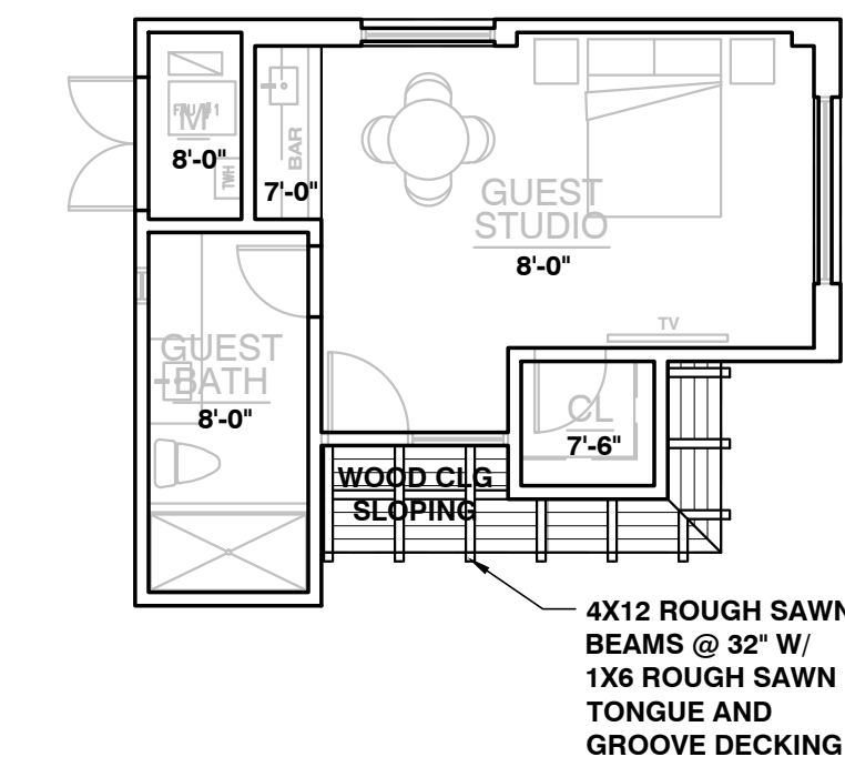
GUEST HOUSE 424 CONCEPT REFLECTED CEILING PLAN
