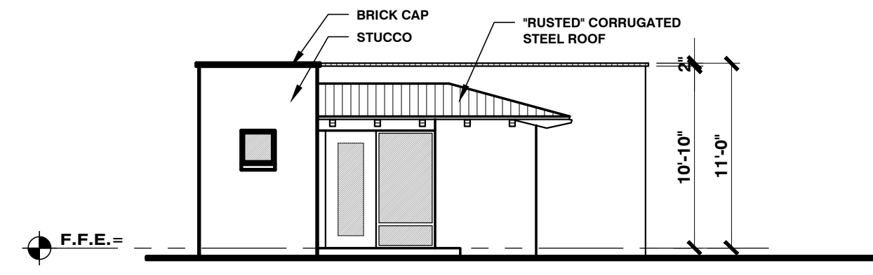
GUEST HOUSE 424 FRONT ELEVATION
