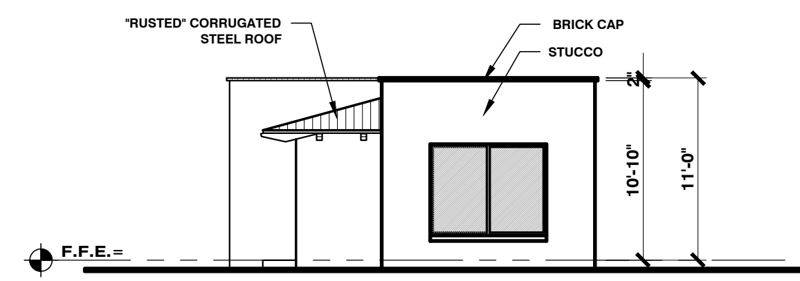
GUEST HOUSE 424 RIGHT ELEVATION
