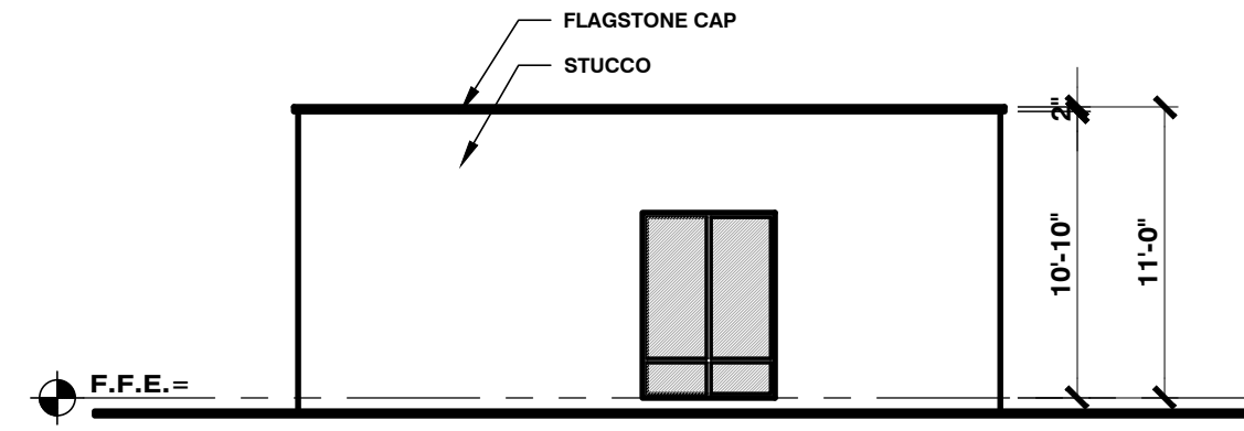
GUEST HOUSE 424 REAR ELEVATION
