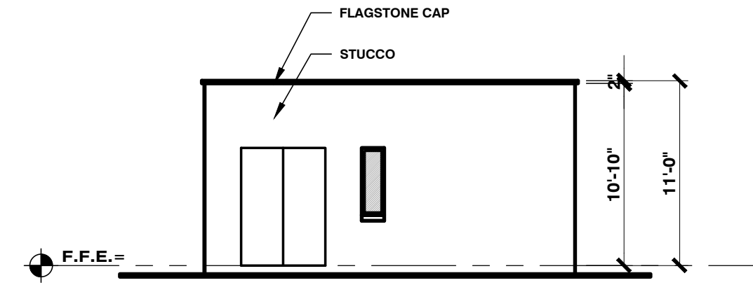
GUEST HOUSE 424 LEFT ELEVATION
