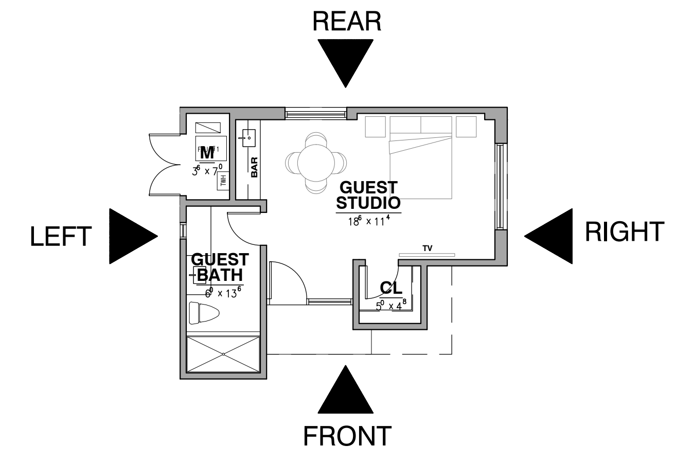
GUEST HOUSE 424 CONCEPT FLOOR PLAN
